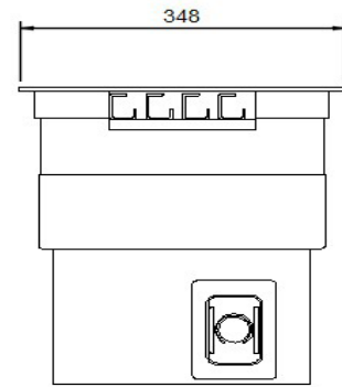
FRONT VIEW NTS
