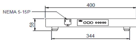
FRONT VIEW NTS
