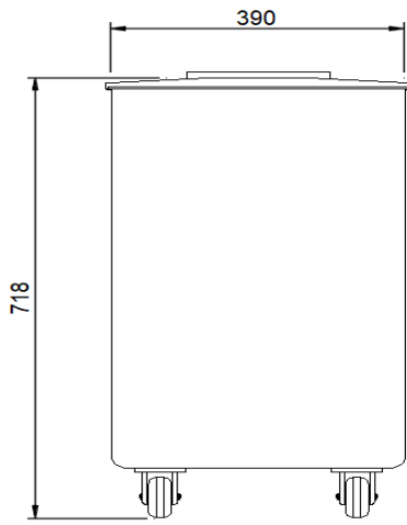
FRONT VIEW NTS
