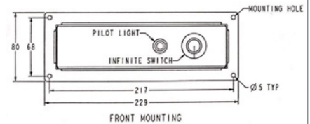
GM5AH Control Box
