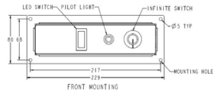
GM5AHL Control Box
