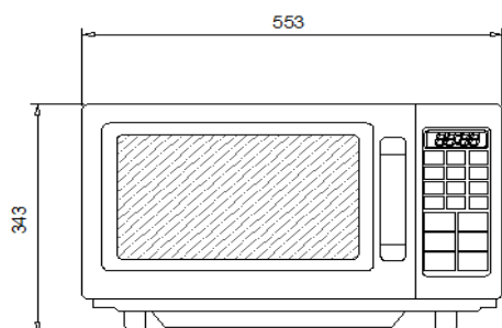
FRONT VIEW NTS
