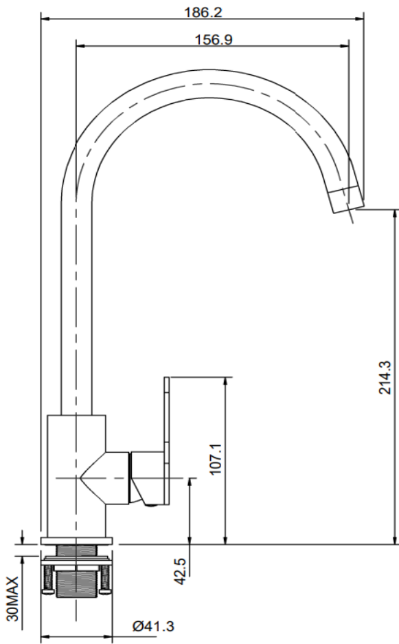
FRONT VIEW NTS
